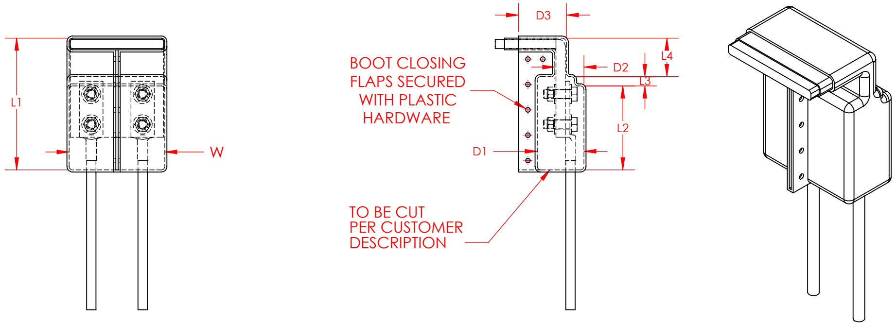
FIGURE 1 (W/ 90° CONNECTION)
