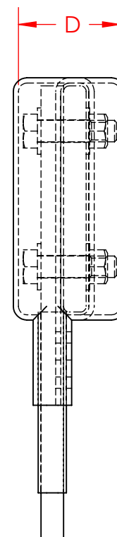
SINGLE RISER
