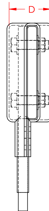
SINGLE RISER
